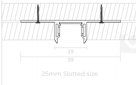
TLS-MS15X0 Trimless Recessed Track
