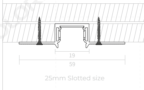
TLS-MR15X0(B) Recessed Track
