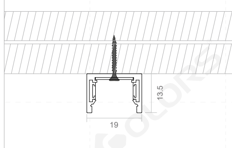
TLS-MS15X0 Ceiling Track
