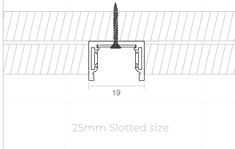
TLS-MS15X0 Trimless Recessed Track
